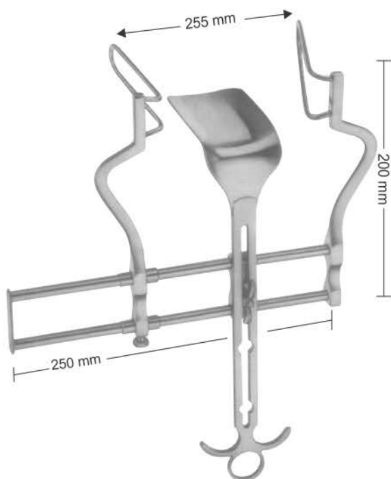
Balfour Retractor ST11-752-00 Lateral blades 105 mm deep Center blade 107 x 59 mm
