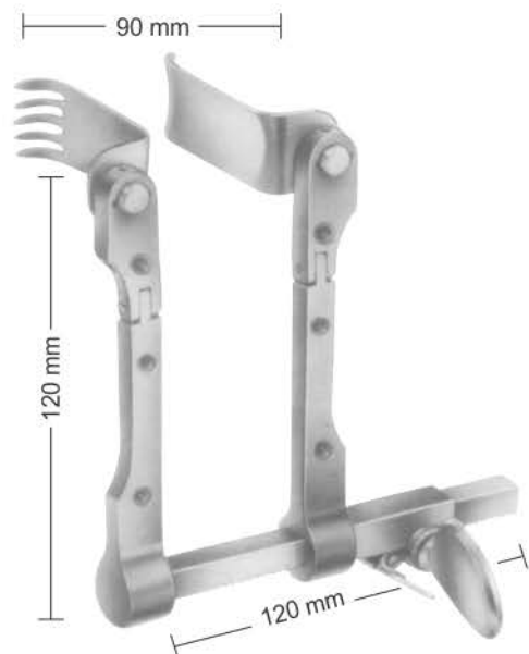
Caspar Retractor ST11-730-00 Retractor, adjustable, consisting of: 5 medial blades, 5 Lateral blades.
