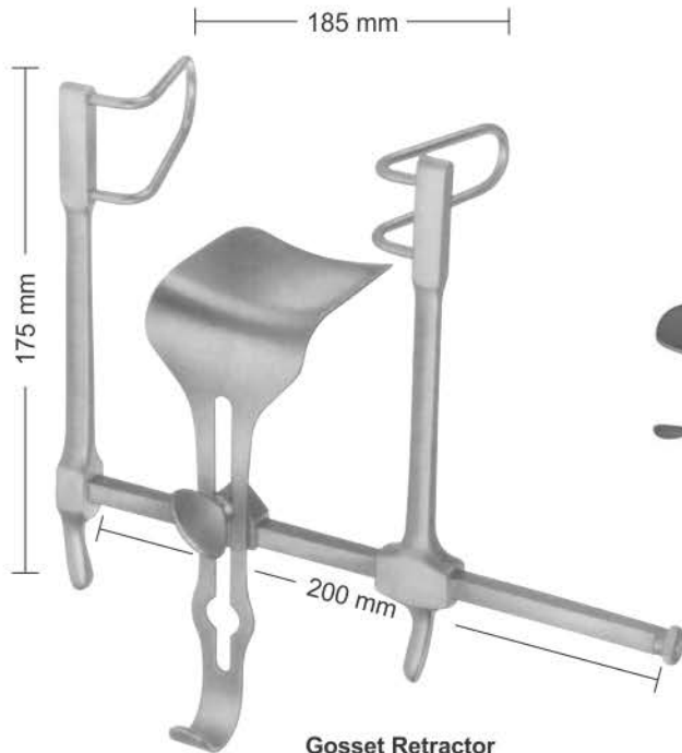
Gosset Retractor ST11-764-00 Lateral Blades 58 mm deep Center blade 59 x 57 mm
