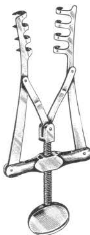
Allport Retractor, ST11-528-10 4x4 semi-sharp prongs, 18mm wide x5mm deep, 40mm spread, total length 10cm
