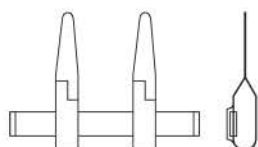
ST22-145-09 x=9mm y=5mm gms=30-40
