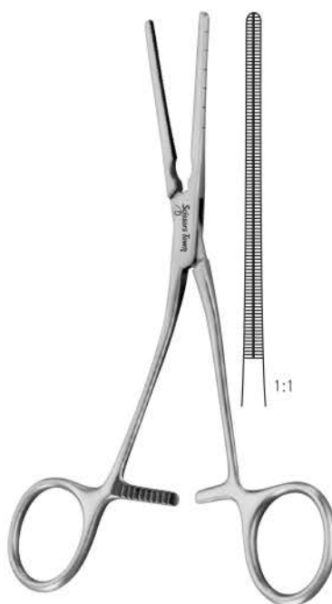
Cooley Patent Ductus Clamp & atraumatic cardiovascular forceps angled on flat, graduated ST22-332-16 16 cm jaw length 3.2 cm angled shanks, calibrated in 5mm increments ST22-332-22 22 cm jaw length 3cm angled shanks, calibrated in 5mm increments
