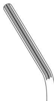
ST22-402-30 17 cm jaw length 3.9 cm angled 30°
