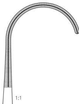
ST22-315-16 16cm ST22-316-20 20 cm jaw length 3.2 cm depth 1.6 cm calibrated in 5mm increments
