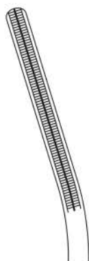
ST22-402-15 17 cm jaw length 3.9 cm angled 15°
